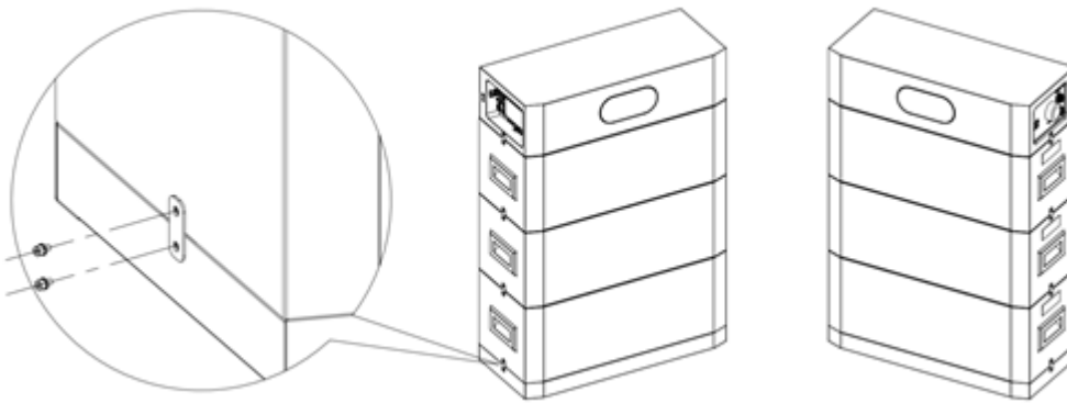
Figure 8 - Schematic diagram of fixing installation
