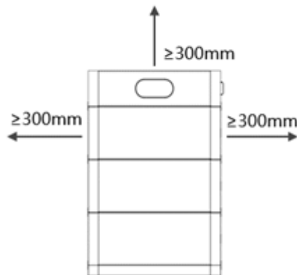
Figure 5 - Installation space diagram
