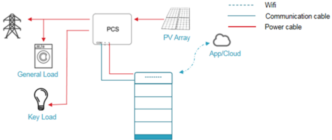
Figure 3 - Single string system diagram
