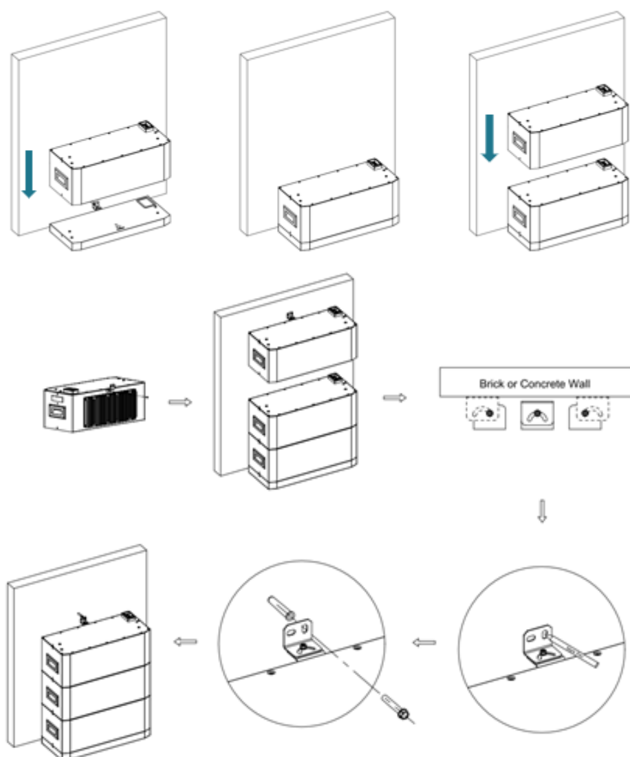
Figure 7 - Battery module installation diagram
