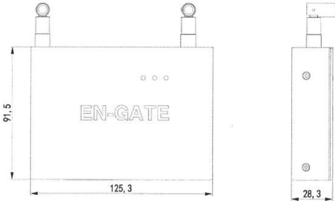
Figure 40 - Device dimensions
