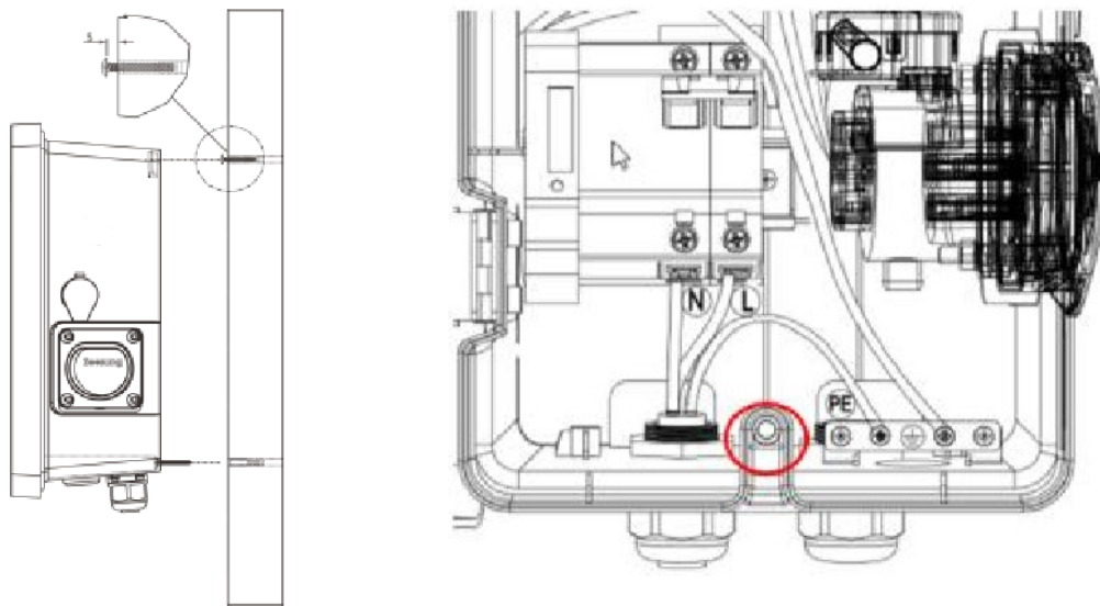
Figure 17 - Wall fixing
