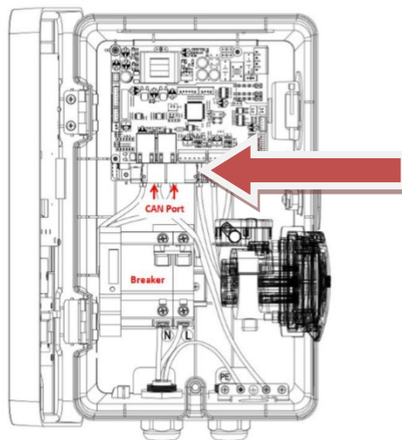
Figure 14 - Communication system
